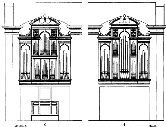
FRONT ELEVATION OF CASES
